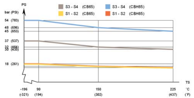
CB65/CBH65 – PED approval pressure/temperature graph
